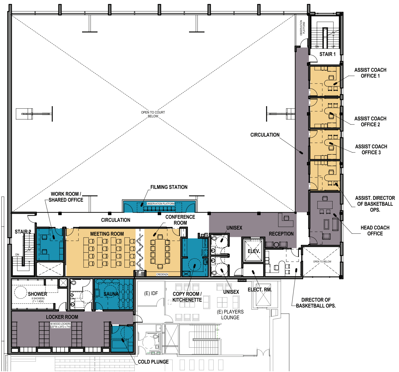
FIRST FLOOR MEZZ. PLAN
